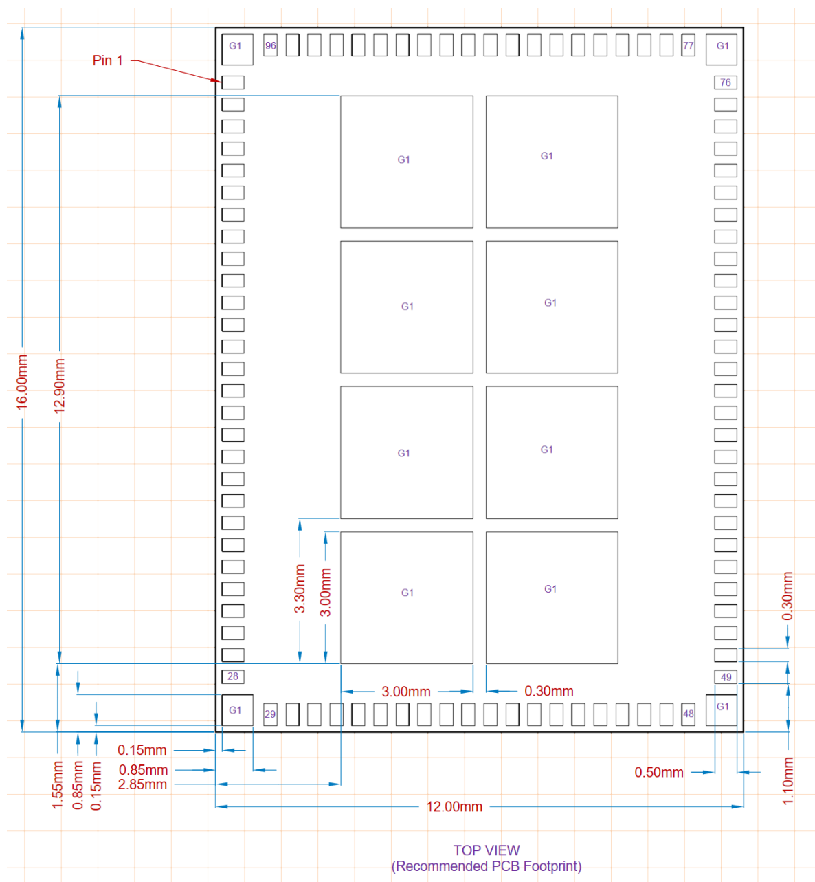
Figure 24: Sona M.2 1216 Footprint
