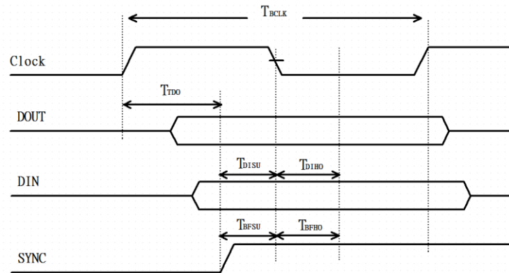
Figure 17: PCM timing specification - slave mode
