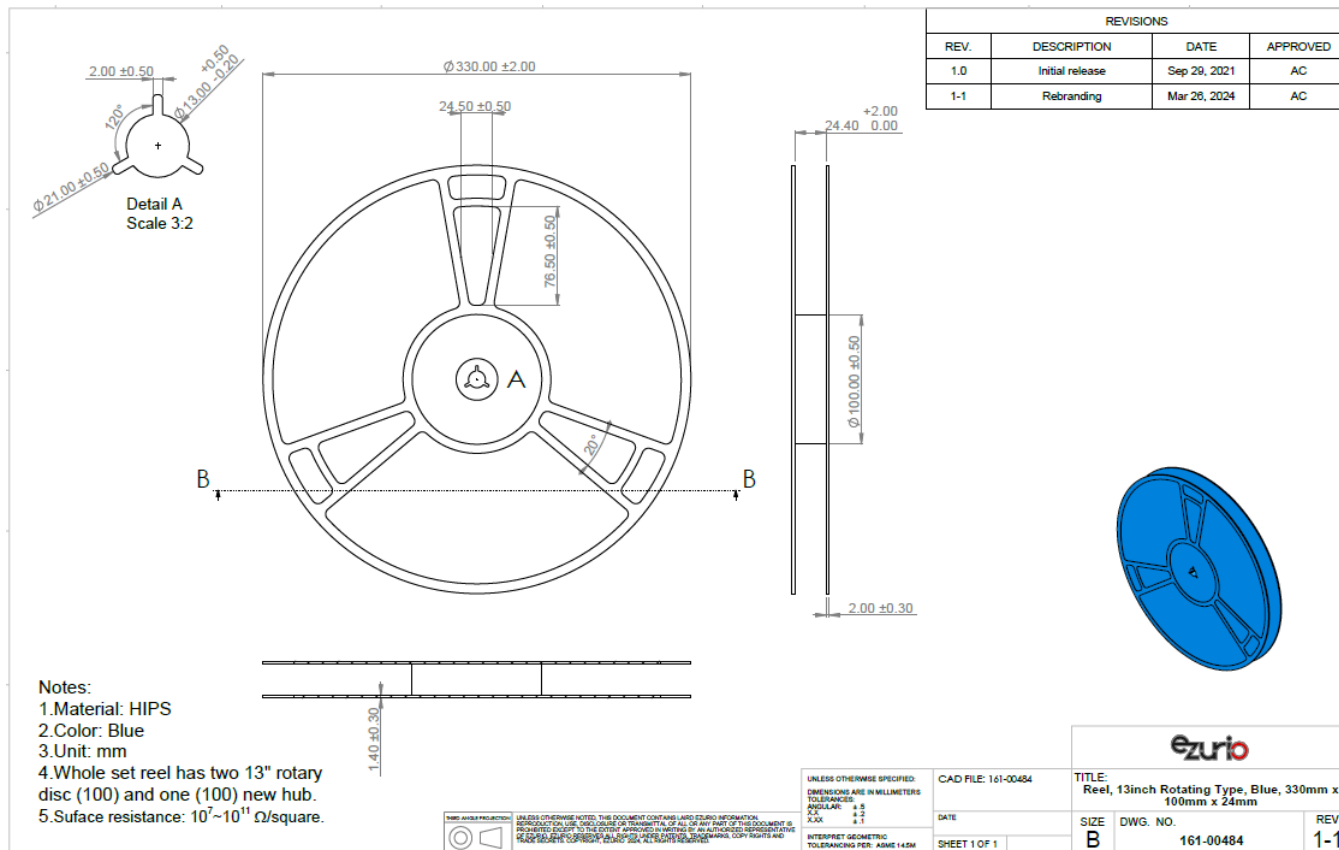
Figure 37: Reel Specification (Sona NX611 1216)
